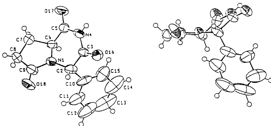
Figure I. Two ORTEP drawings of 16a
